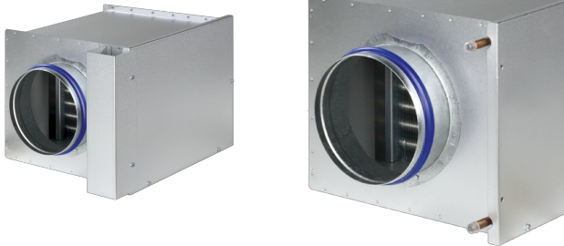
Heat exchanger with copper tubes and aluminium fins
